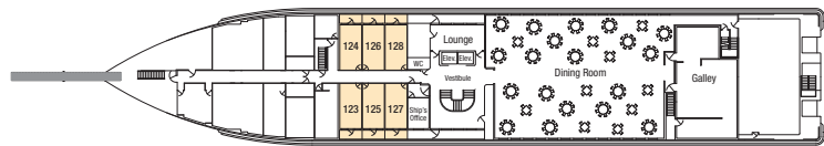
MAIN DECK
